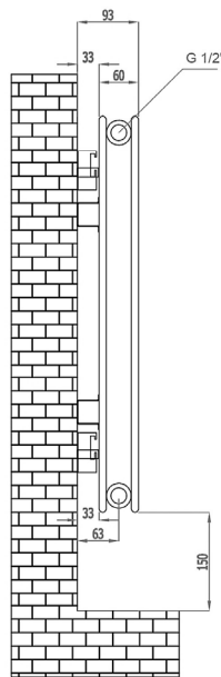
Horizontal Installation
