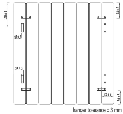
Horizontal Installation
