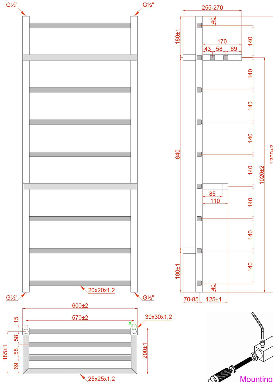
Launton Technical Drawing ( 61.0063 - 61.0065 - 61.0067 )
