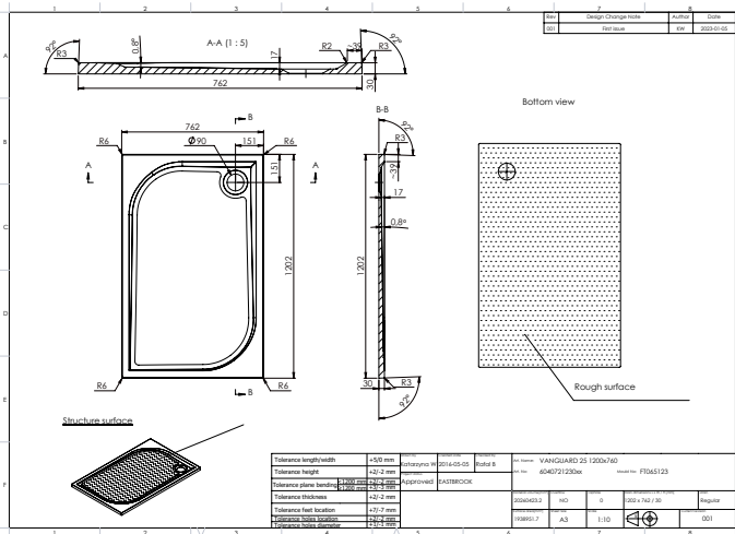
Tray Plan:
