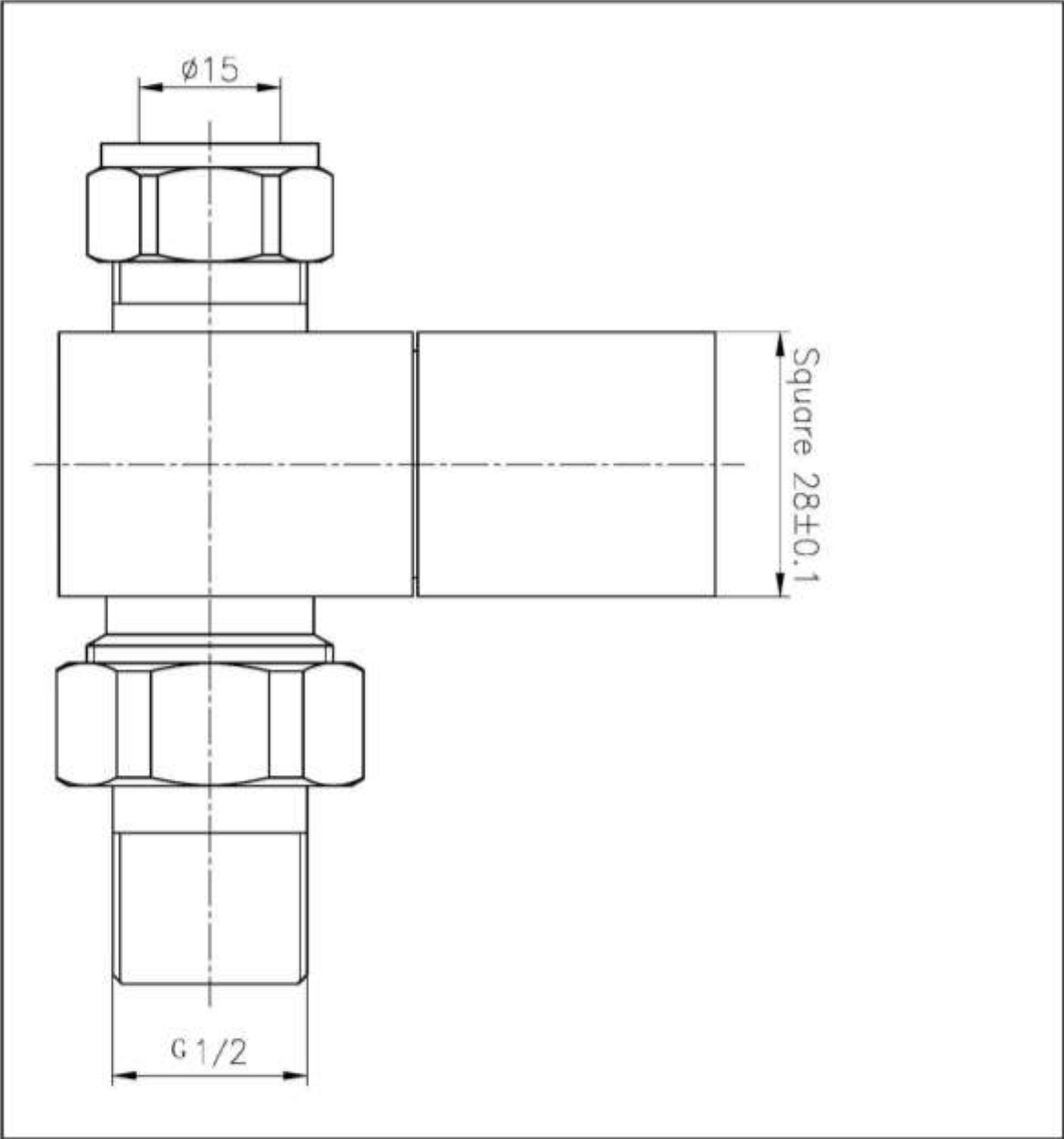
12.039 Straight square radiator valve Brushed Nickel
