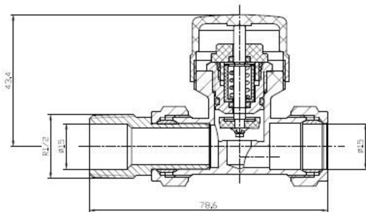
body of TRV
