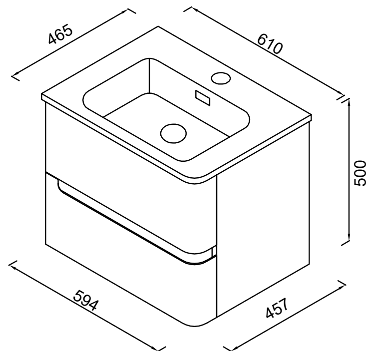
Right Hand Arda Wall hung unit
