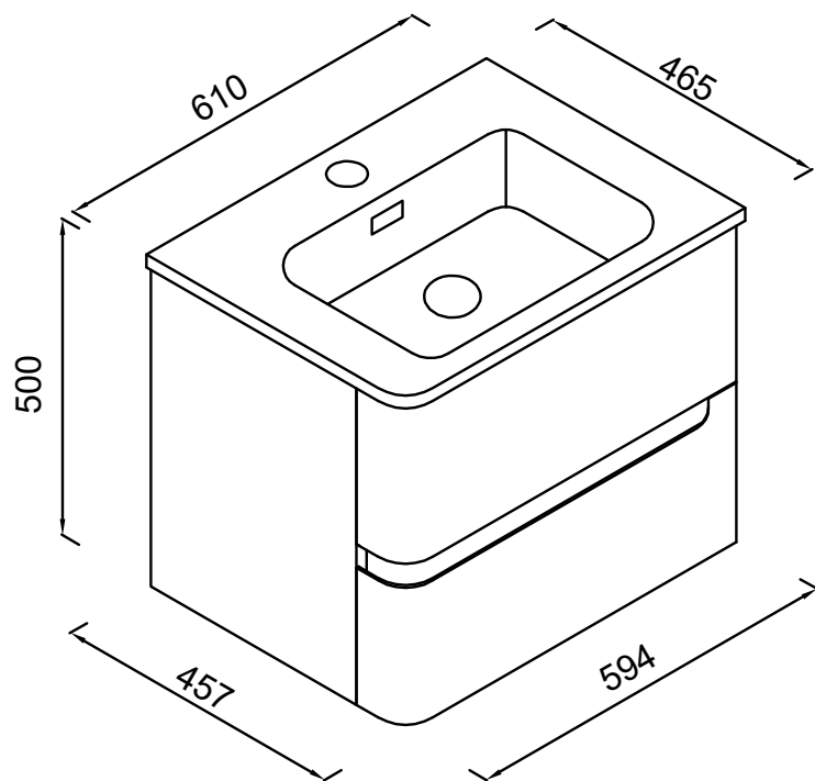
Left Hand Arda Wall hung unit
