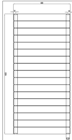
Horizontal Installation
