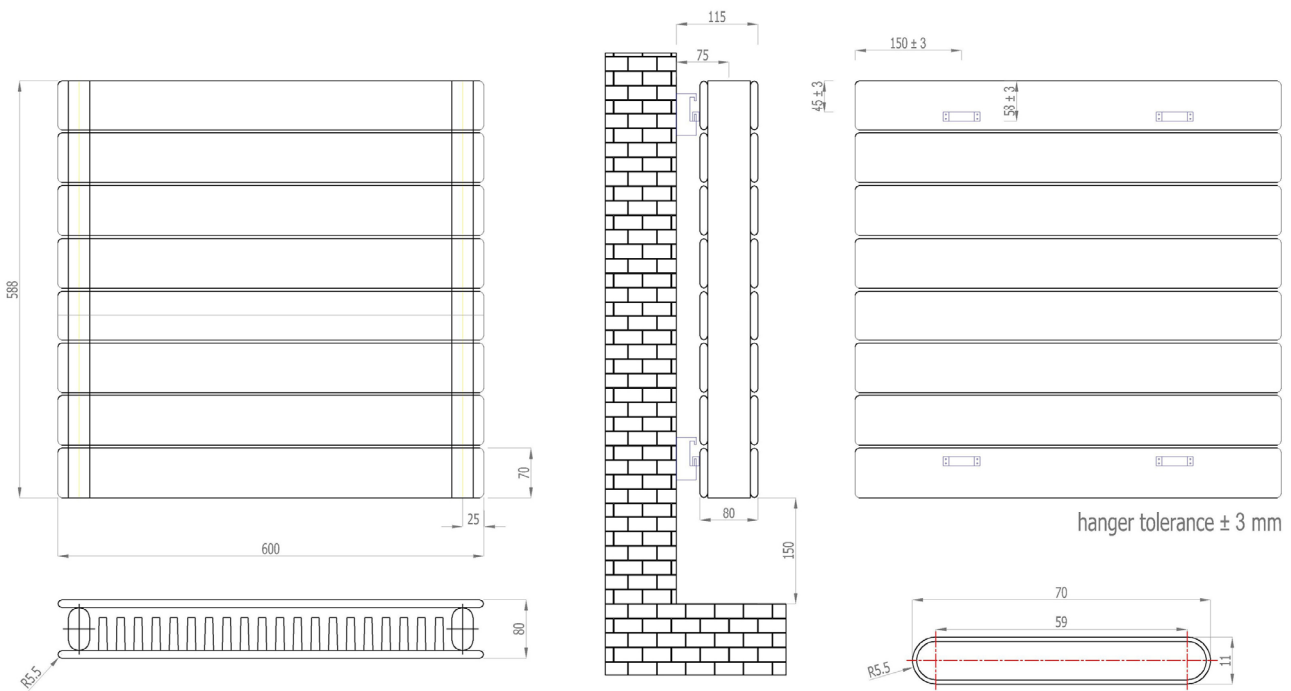
Addington Type21 588 x 600 mm
