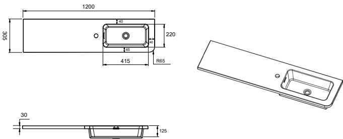
Arda 120cm Polymarble Basin Top RH (37.2095)
