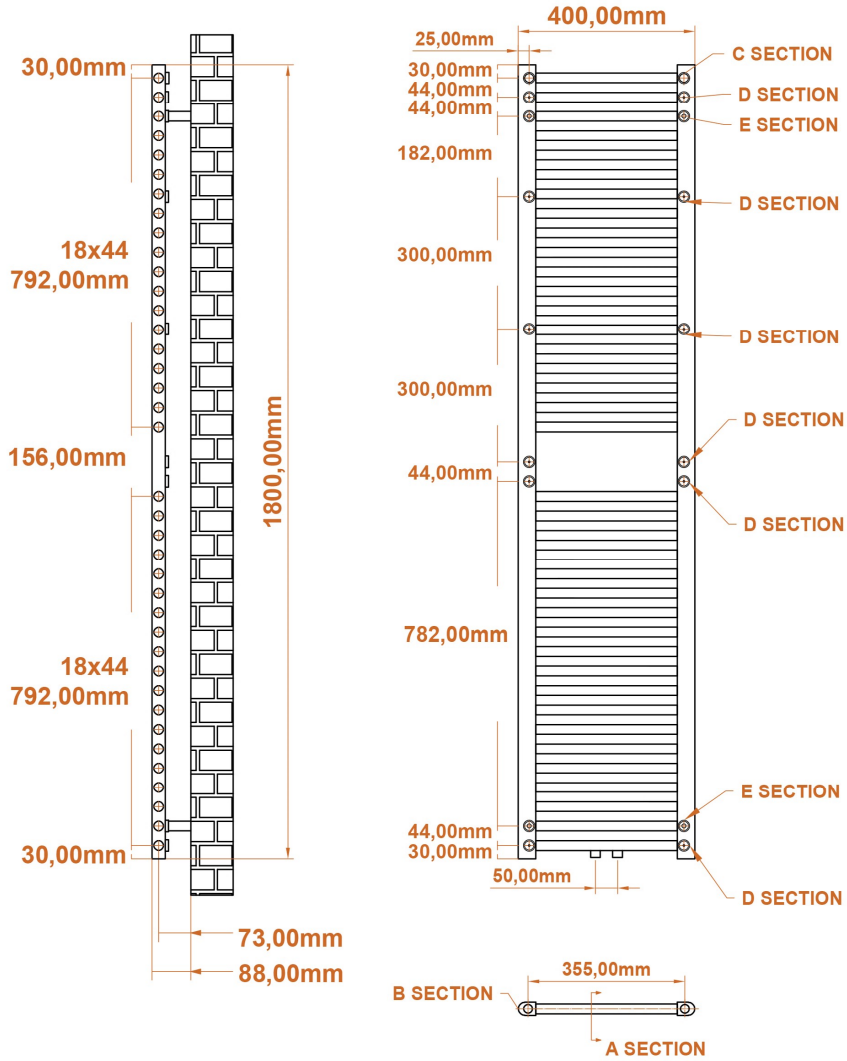
A SECTION
