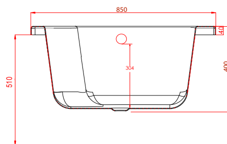
SECTION K-K SCALE 1 : 4
