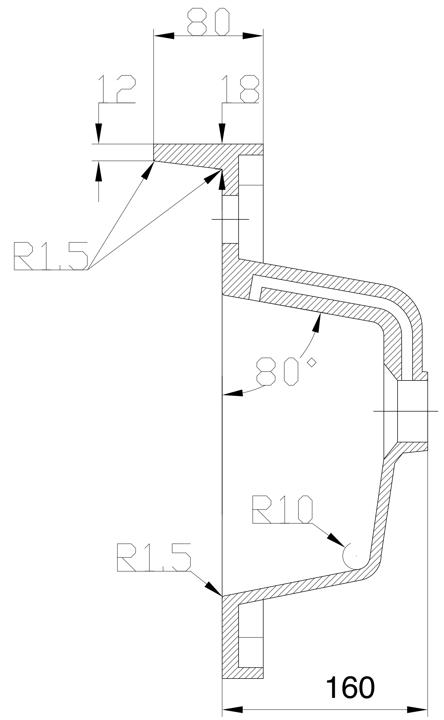
SECTION B-B
