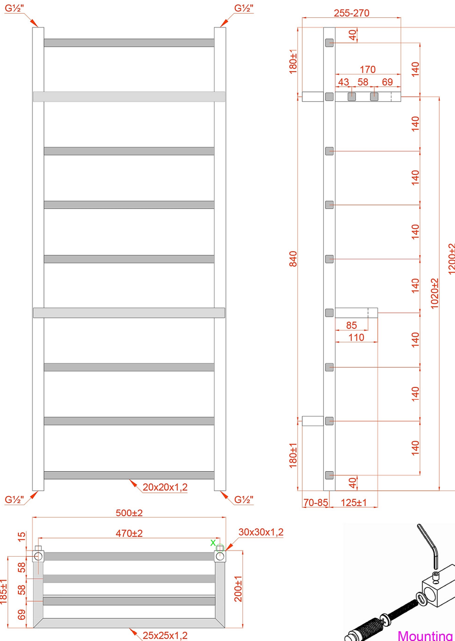
Launton Technical Drawing ( 61.0062 - 61.0064 - 61.0066 )
