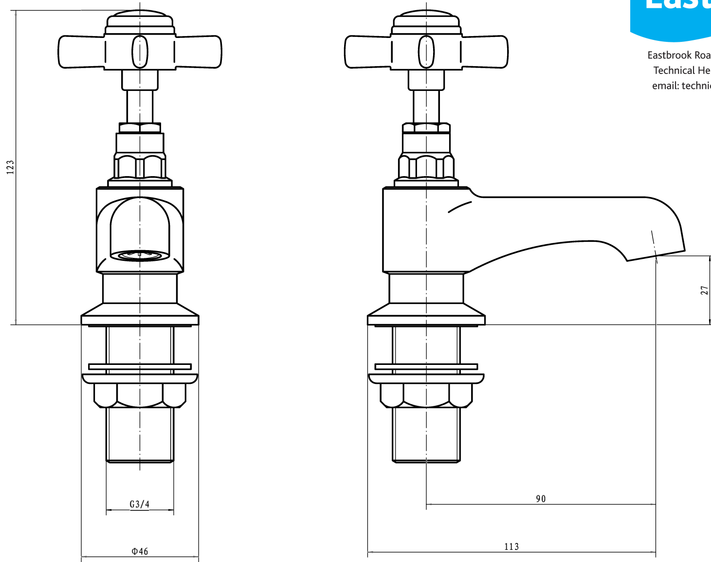
Haymarket Bath Taps
