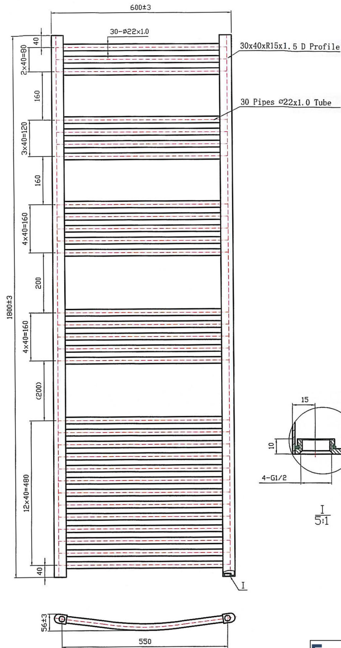
1800*600 30 pipes Curved
