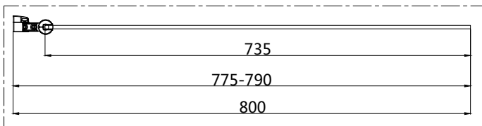
49.0106 6mm curved bath screen 800 x 1400 Chrome
