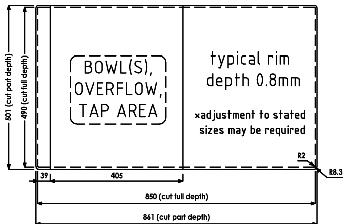
FLUSH MOUNT CUT OUT
