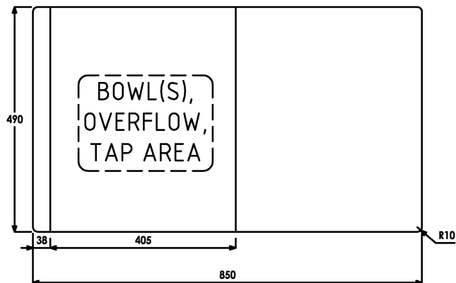
INSET CUT OUT
