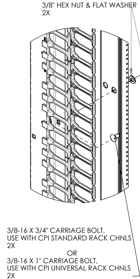
DETAIL B
