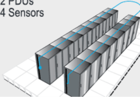
Figure 10: CPI eConnect PDU integrates power monitoring, environmental monitoring and access control into a single system. Integrated Secure Array IP Consolidation technology allows up to 32 PDUs and all attached sensors and locks to share a single network connection significantly reducing networking costs.
