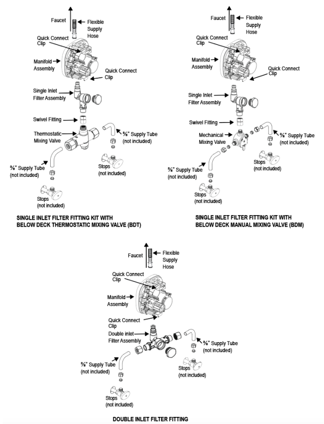
DOUBLE INLET FILTER FITTING
