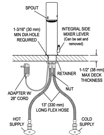
EFX-100.50X.0X1X Faucet with Hot & Cold Water Supply
