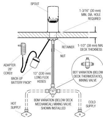
EFX-300.X0X.0X1X Faucet with Hot & Cold Water Supply
