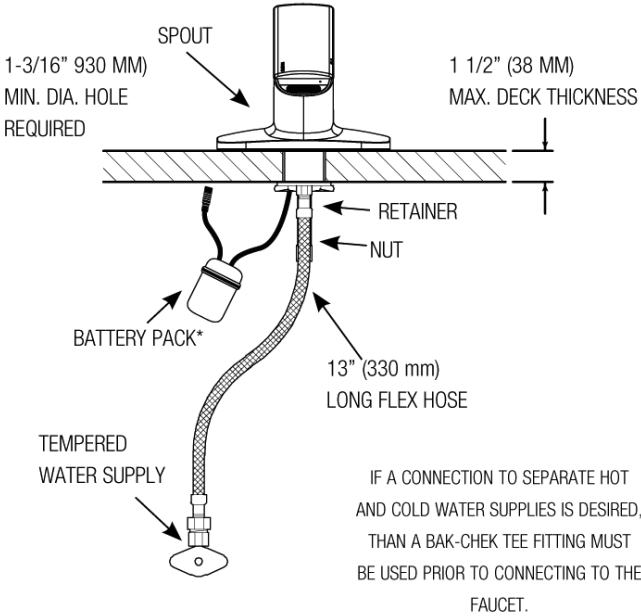
EFX-650.X0X.0000 Faucet with single line water supply
