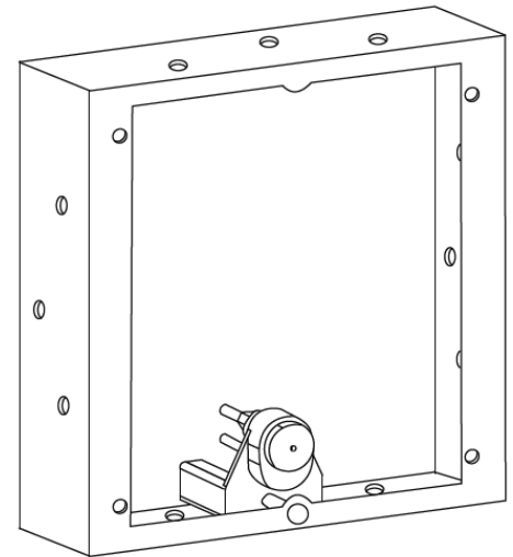
PROPER WALL FRAME ORIENTATION
