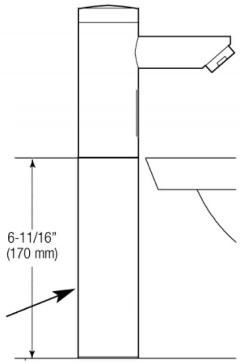
Optional EAF-35-A Faucet Extension Kit
