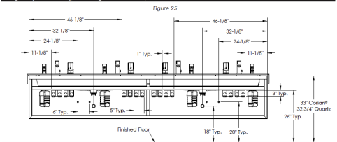
Rough-In (Four Station): Plumbing and Electrical, front View
