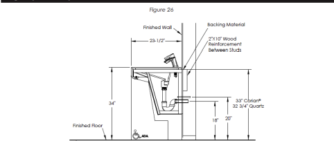
Rough-In (Four Station): Section View
