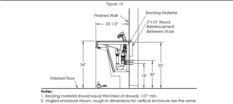
Rough-In (Two Station): Section View
