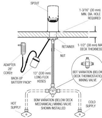
EFX-300.X0X.0X1X Faucet with Hot & Cold Water Supply
