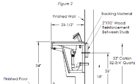
Rough-in (One Station): Section View
