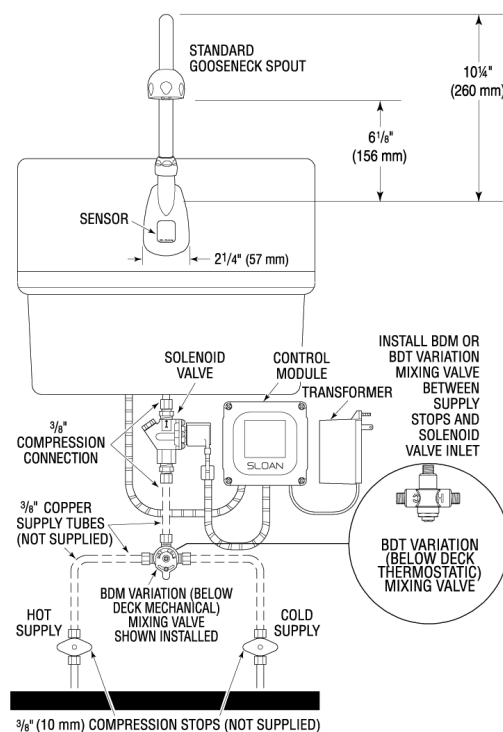
ETF-500 Faucet with BDM and BDT Variation Mixing Valves for Hot and Cold Water Supply
