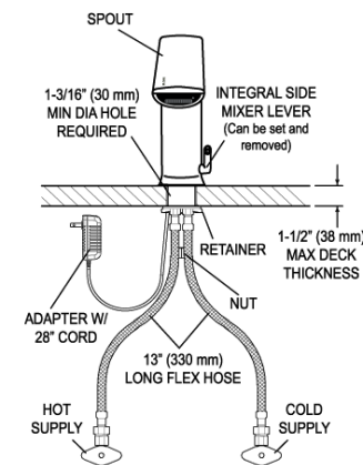
EFX-200.50X.0X1X Faucet with Hot & Cold Water Supply
