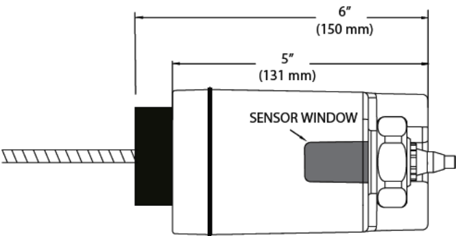
Side Mount Hardwired Unit Dimensions
