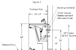
Rough-in (One Station): Section View
