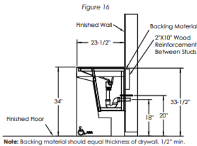
Rough-In (Three Station): Section View
