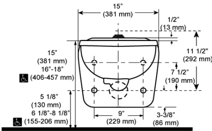
Designed to meet ADA standards when bowl is 17" - 19" high including seat
