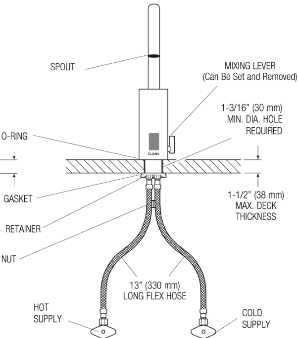
EAF-700-ISM Faucets with Hot and Cold Water Supply
