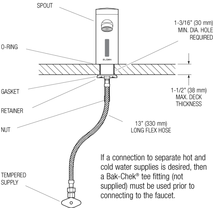
EAF-200 Faucets with Single Line Water Supply
