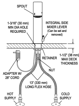
EFX-100.50X.0X1X Faucet with Hot & Cold Water Supply
