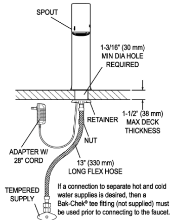
EFX-100.00X.0X1X Faucet with Single Line Water Supply
