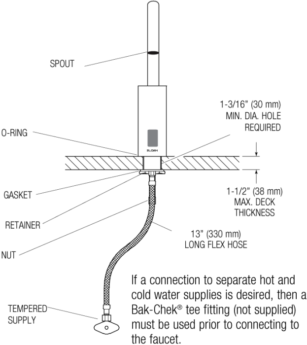
EAF-700 Faucets with Single Line Water Supply
