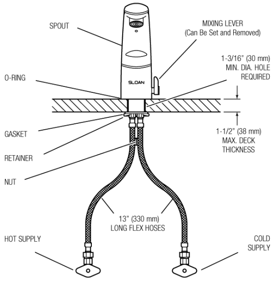
EAF-100-ISM, EAF-100-ISM-IC AND EAF-100-ISM-DPU-IC Faucets with Hot and Cold Water Supply
