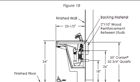
Rough-In (Three Station); Section View
