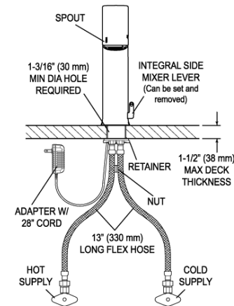
EFX-100.50X.0X1X Faucet with Hot & Cold Water Supply
