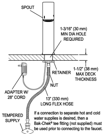
EFX-100.00X.0X1X Faucet with Single Line Water Supply
