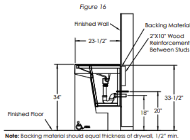
Rough-In (Three Station): Section View
