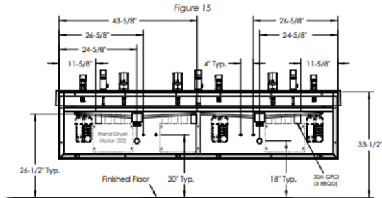
Rough-In (Three Station): Plumbing and Electrical, Front View
