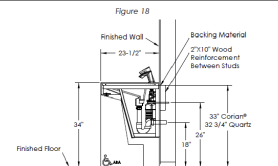
Rough-in (Three Station): Section View
