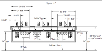
Rough-in (Three Station): Plumbing and Electrical, Front View
