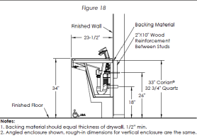
Rough-in (Three Station): Section View
