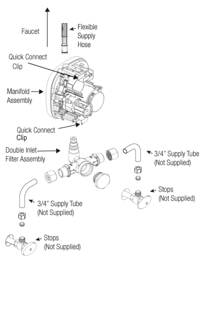
Double Inlet Filter Fitting
