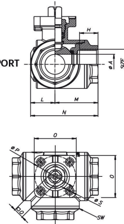
3-way ball valve, full bore with T-port .
