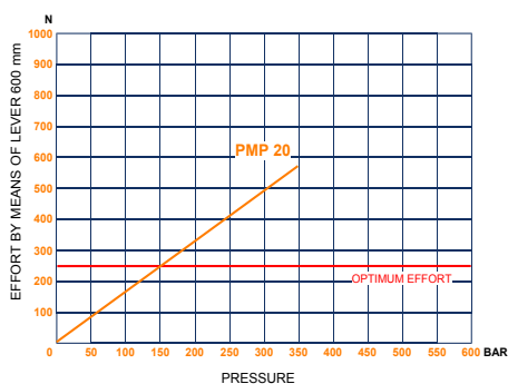
EFFORT DIAGRAM pin in D (distance between centers: 40 mm)
